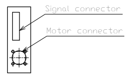
A-view (S=1/5)
